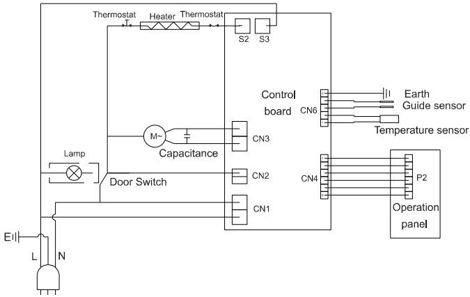
Electric diagram
